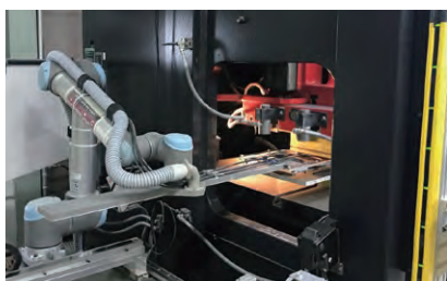
社内運用プレス加工自動供給ロボット Automatic supply robot in in-house operation for pressing process
